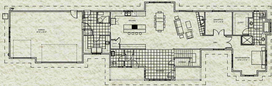
1st Floor Plan
